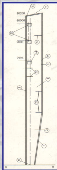
MAIN COLUMN ( C - 1 ) QTY. = 4 NOS.
